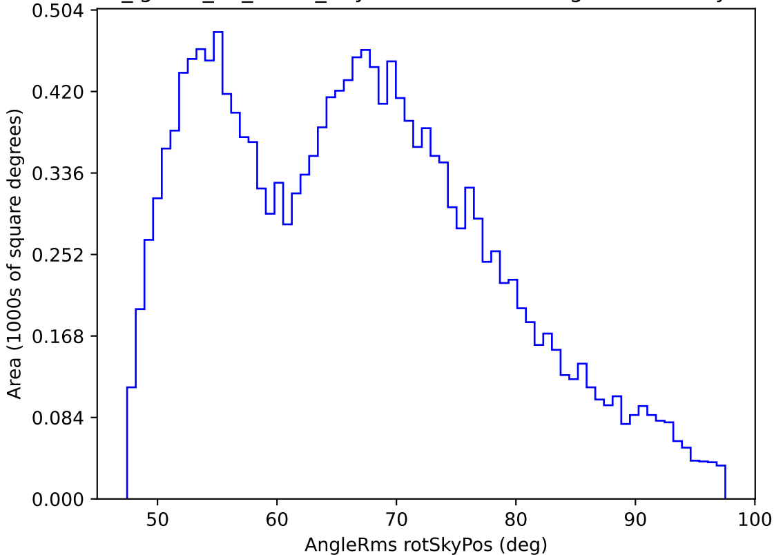
too_ignore_10_4v3.4_10yrs WFD r band: AngleRms rotSkyPos
