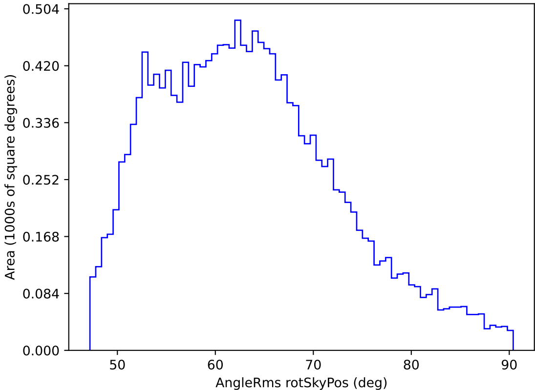
too_ignore_10_4v3.4_10yrs WFD i band: AngleRms rotSkyPos
