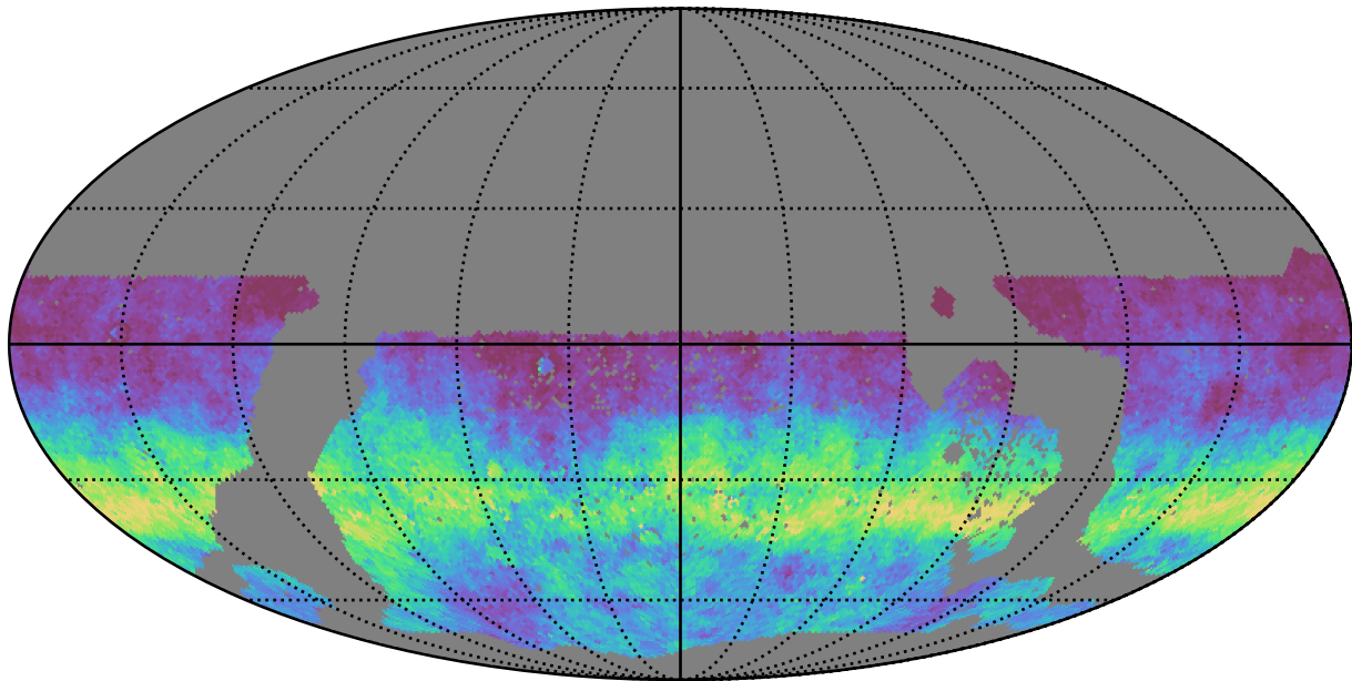
too_ignore_10_4v3.4_10yrs WFD g band: AngleRms rotSkyPos
