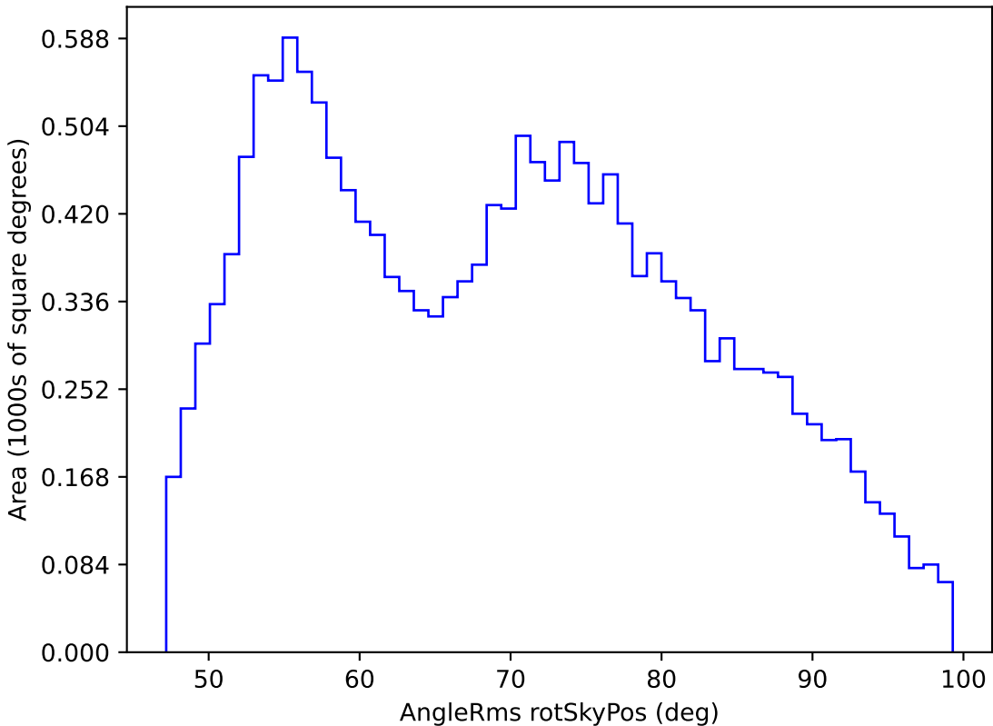
too_ignore_10_4v3.4_10yrs WFD g band: AngleRms rotSkyPos
