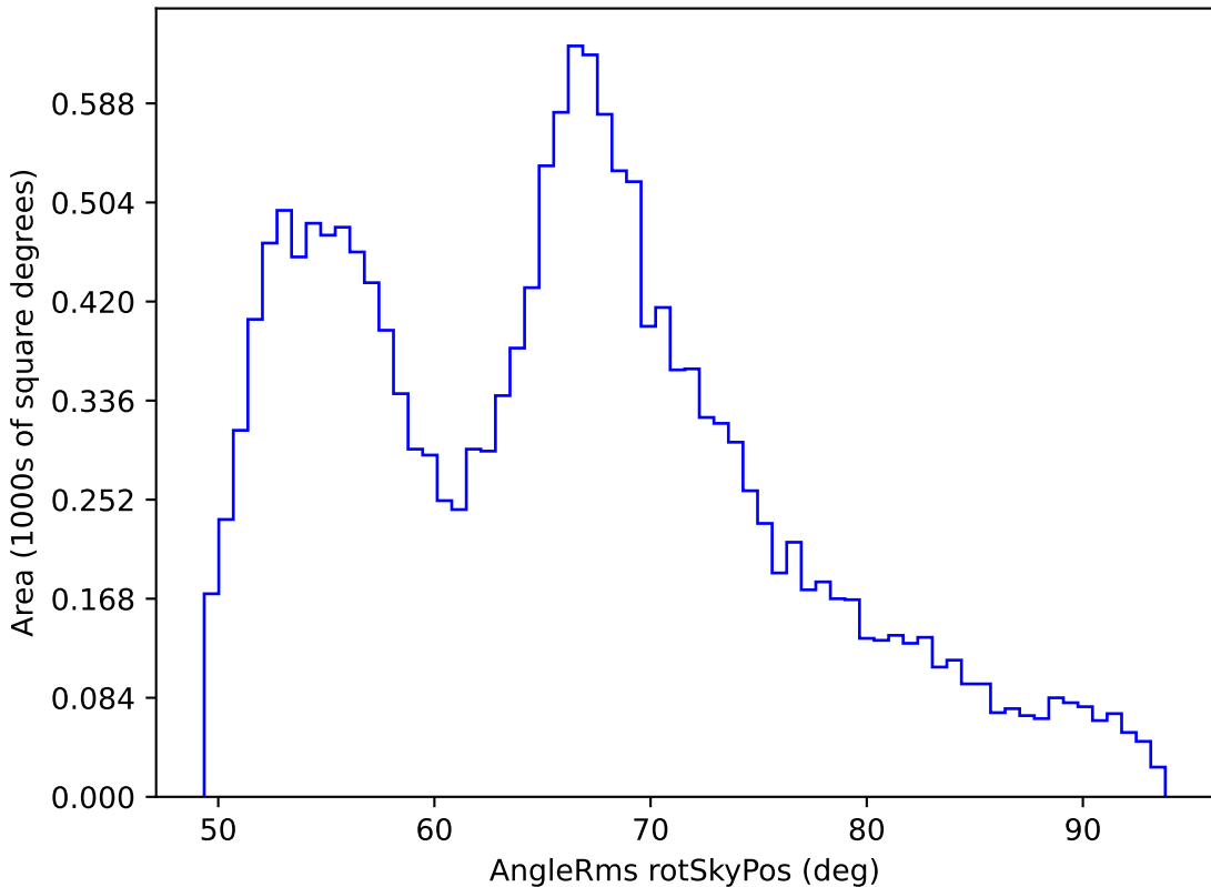
too_ignore_10_4v3.4_10yrs WFD all bands: AngleRms rotSkyPos
