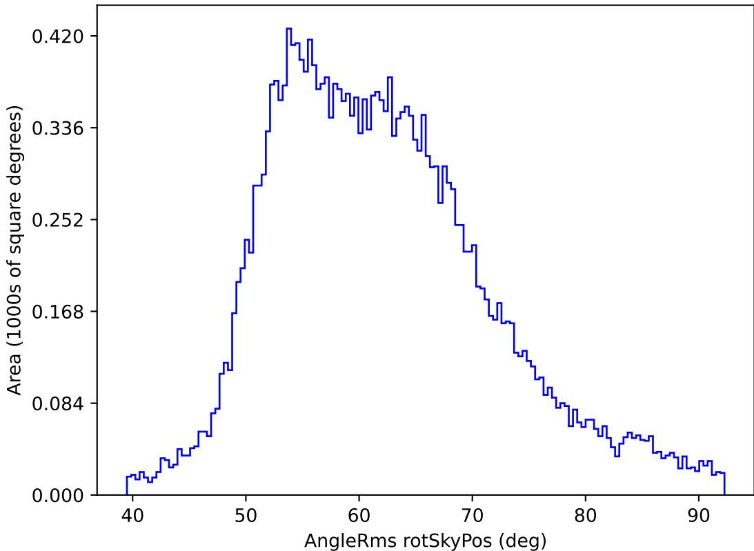
too_ignore_10_4v3.4_10yrs All sky y band: AngleRms rotSkyPos
