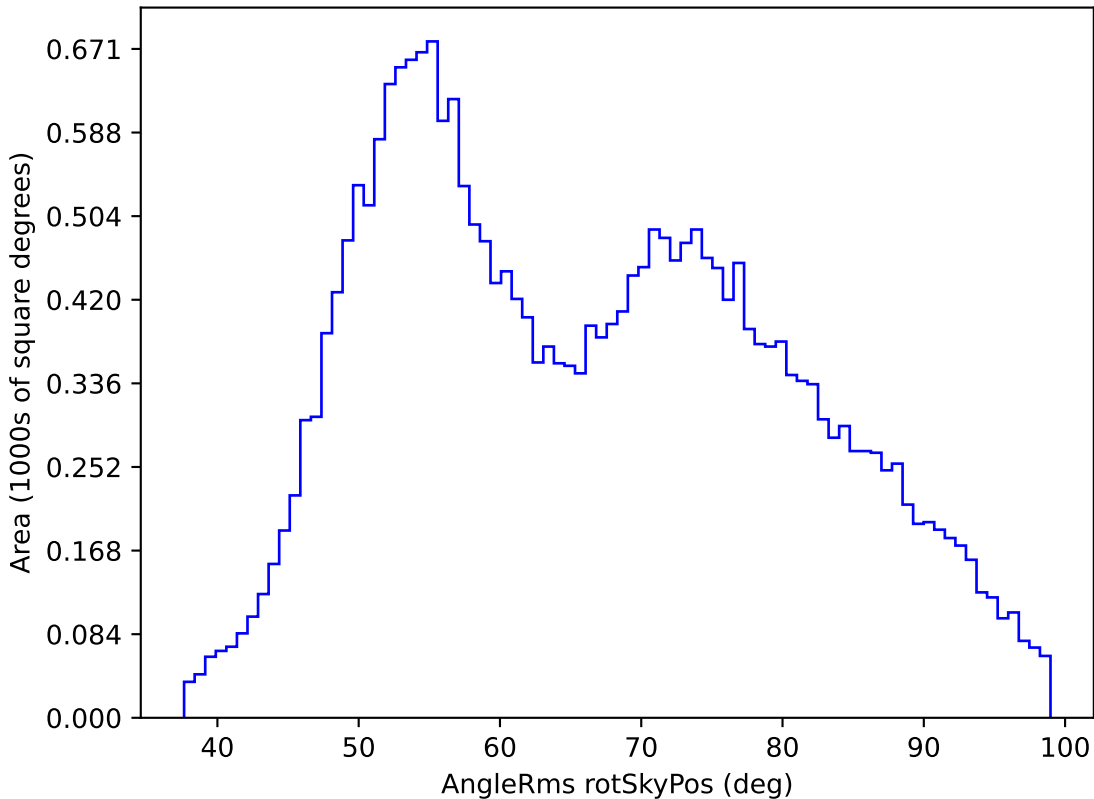
too_ignore_10_4v3.4_10yrs All sky g band: AngleRms rotSkyPos
