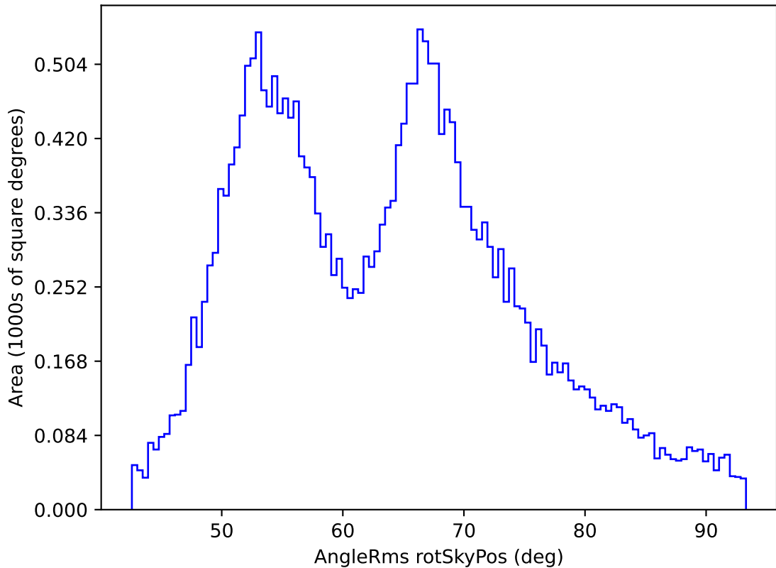
too_ignore_10_4v3.4_10yrs All sky all bands: AngleRms rotSkyPos
