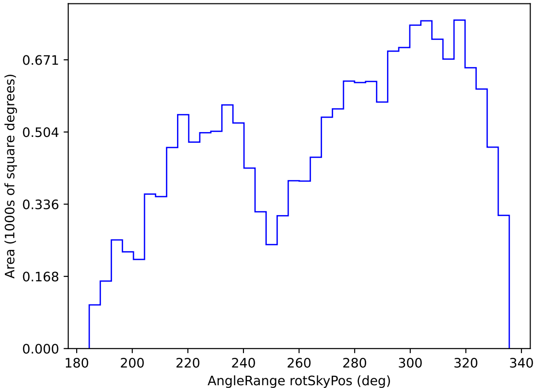
too_ignore_10_4v3.4_10yrs WFD g band: AngleRange rotSkyPos
