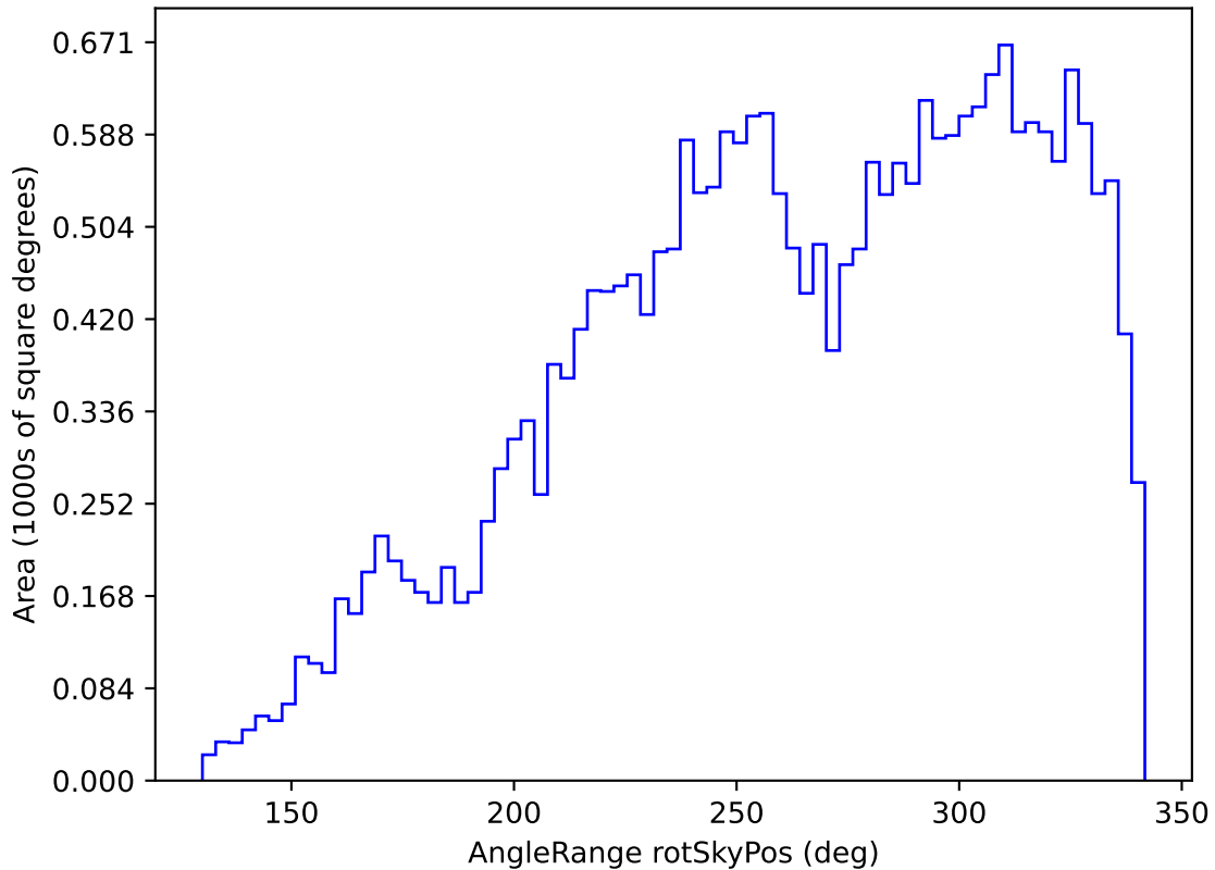
too_ignore_10_4v3.4_10yrs All sky z band: AngleRange rotSkyPos
