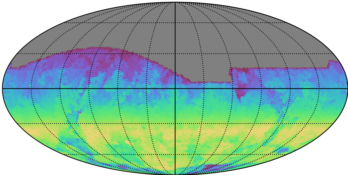
too_ignore_10_4v3.4_10yrs All sky r band: AngleRange rotSkyPos
