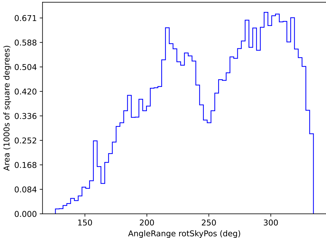
too_ignore_10_4v3.4_10yrs All sky g band: AngleRange rotSkyPos
