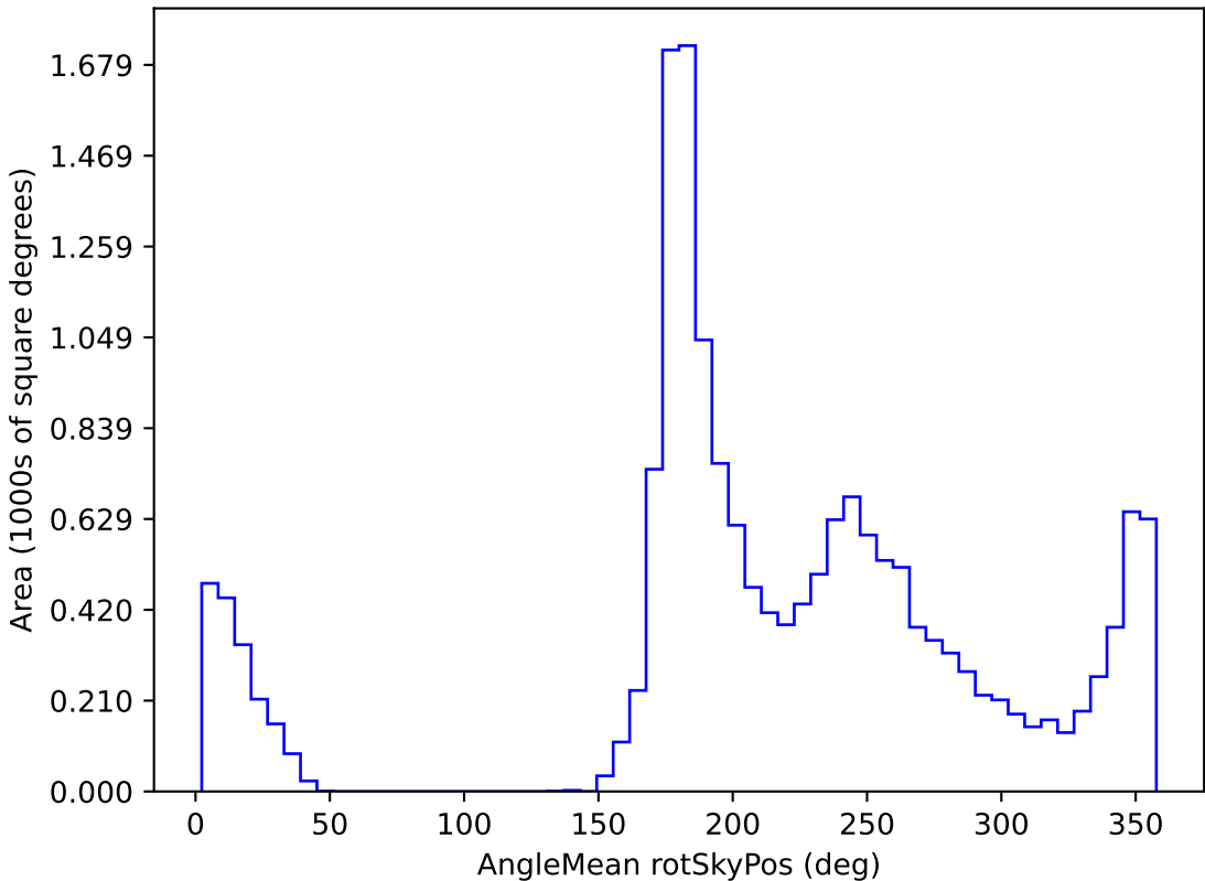
too_ignore_10_4v3.4_10yrs WFD z band: AngleMean rotSkyPos
