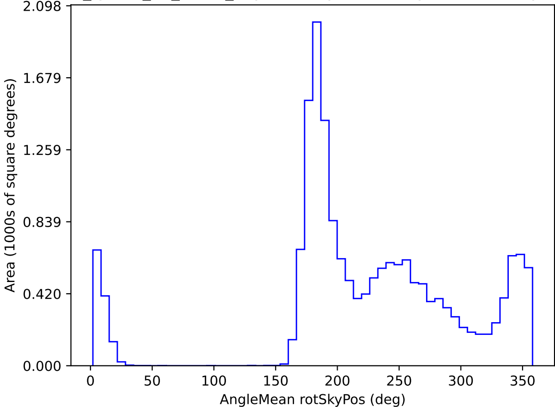
too_ignore_10_4v3.4_10yrs WFD y band: AngleMean rotSkyPos
