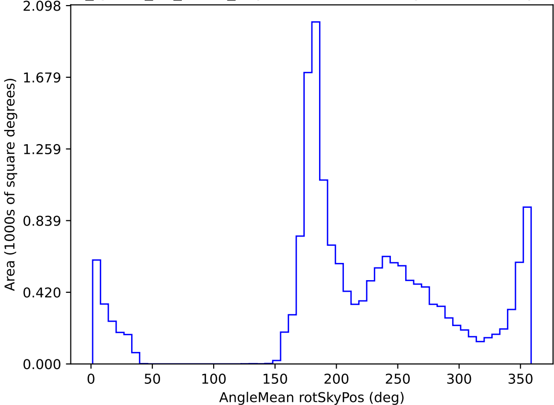
too_ignore_10_4v3.4_10yrs WFD i band: AngleMean rotSkyPos
