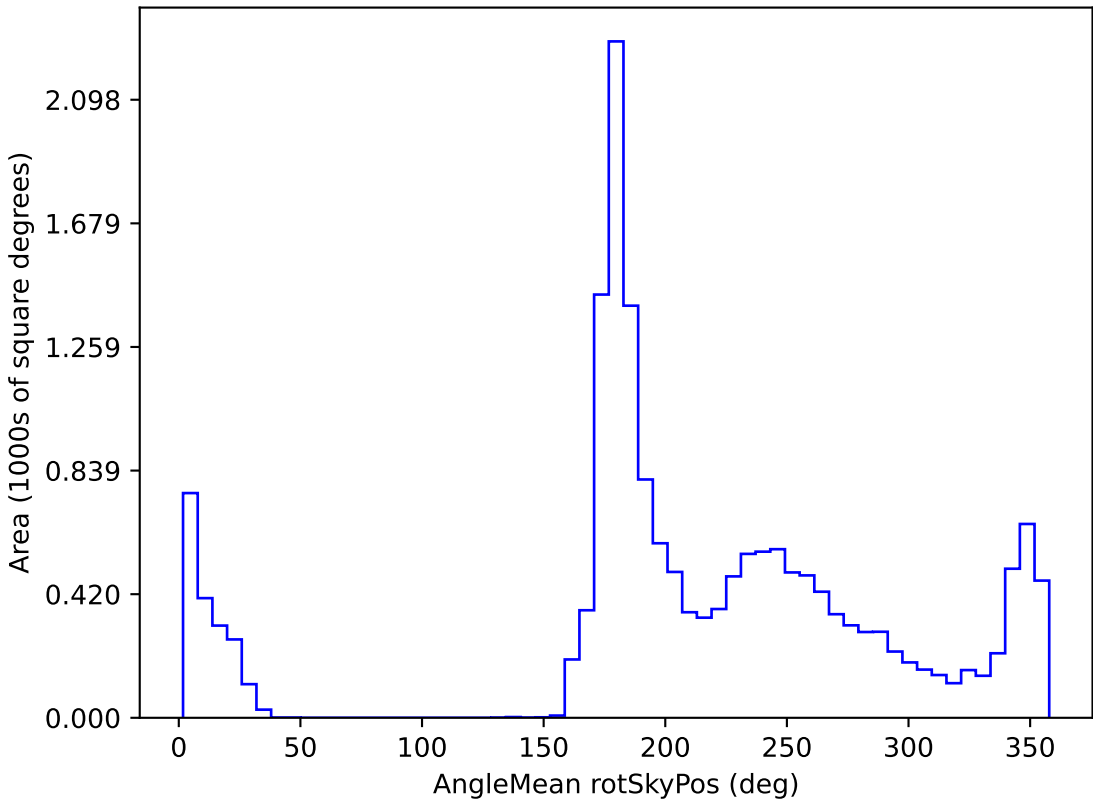
too_ignore_10_4v3.4_10yrs WFD all bands: AngleMean rotSkyPos
