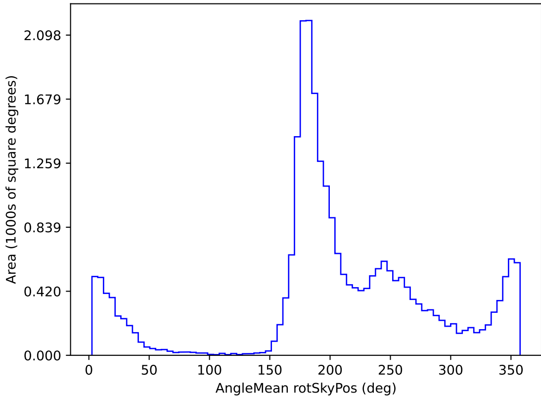
too_ignore_10_4v3.4_10yrs All sky z band: AngleMean rotSkyPos
