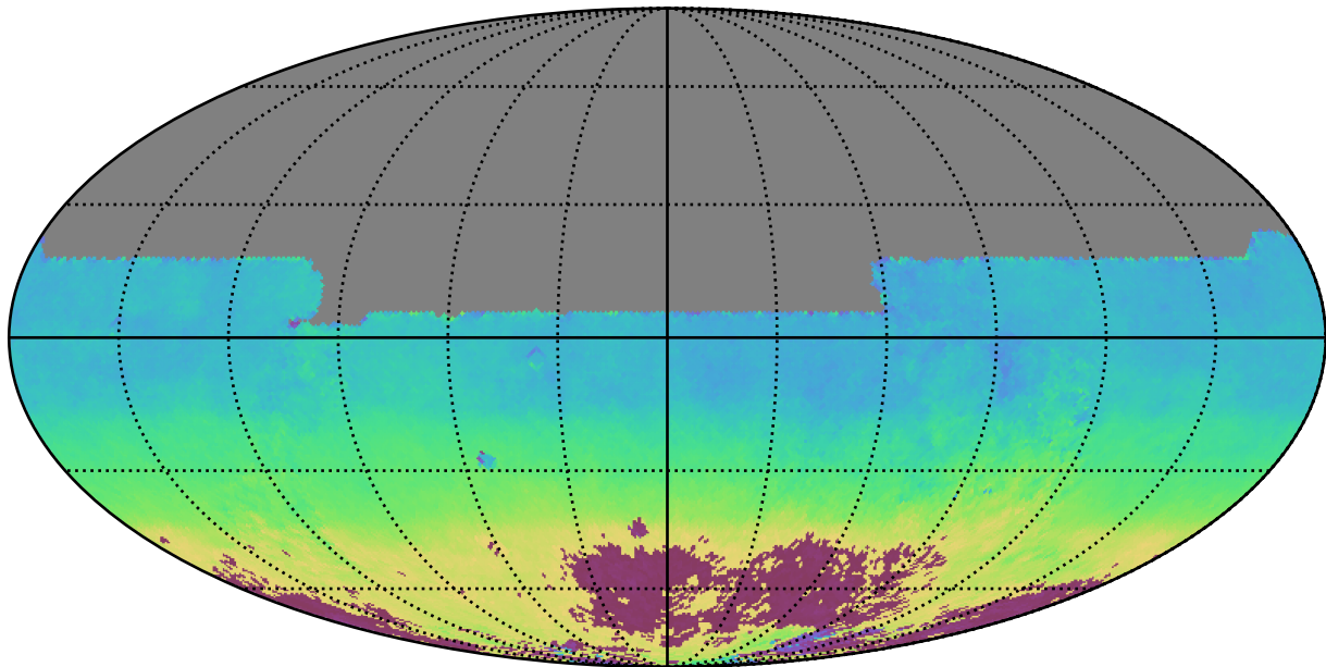
too_ignore_10_4v3.4_10yrs All sky y band: AngleMean rotSkyPos
