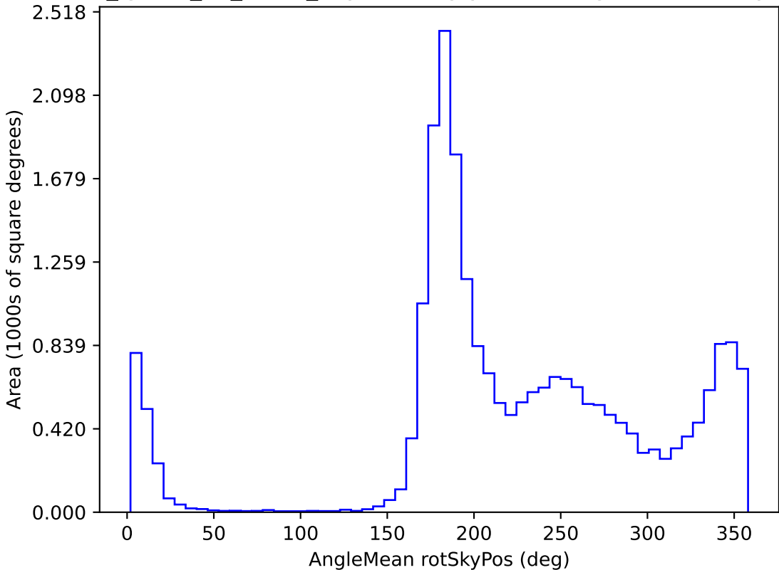
too_ignore_10_4v3.4_10yrs All sky y band: AngleMean rotSkyPos
