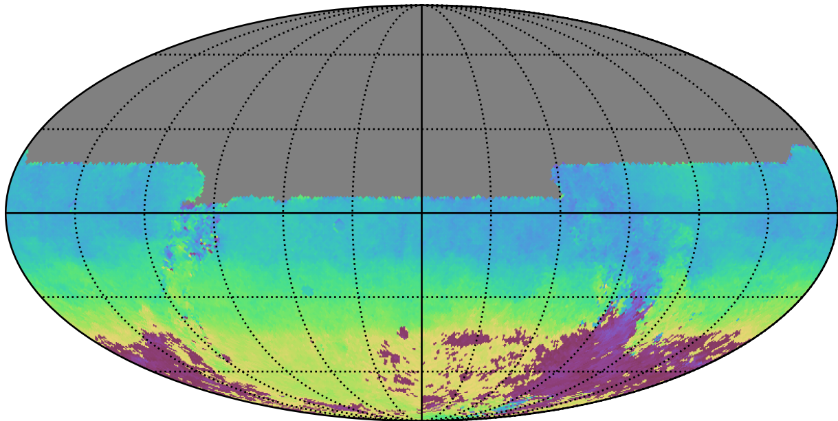
too_ignore_10_4v3.4_10yrs All sky u band: AngleMean rotSkyPos
