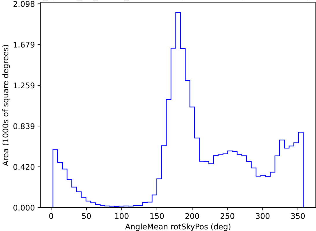
too_ignore_10_4v3.4_10yrs All sky u band: AngleMean rotSkyPos
