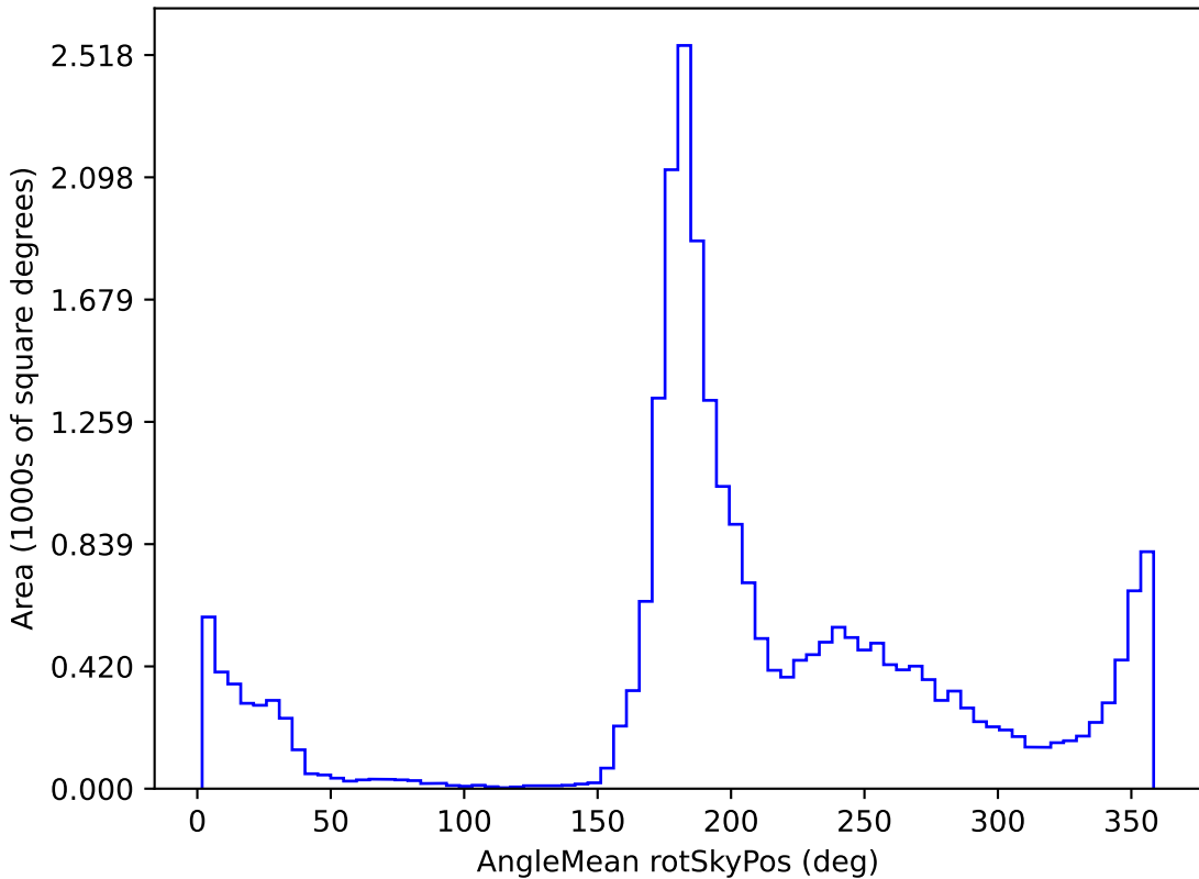
too_ignore_10_4v3.4_10yrs All sky i band: AngleMean rotSkyPos
