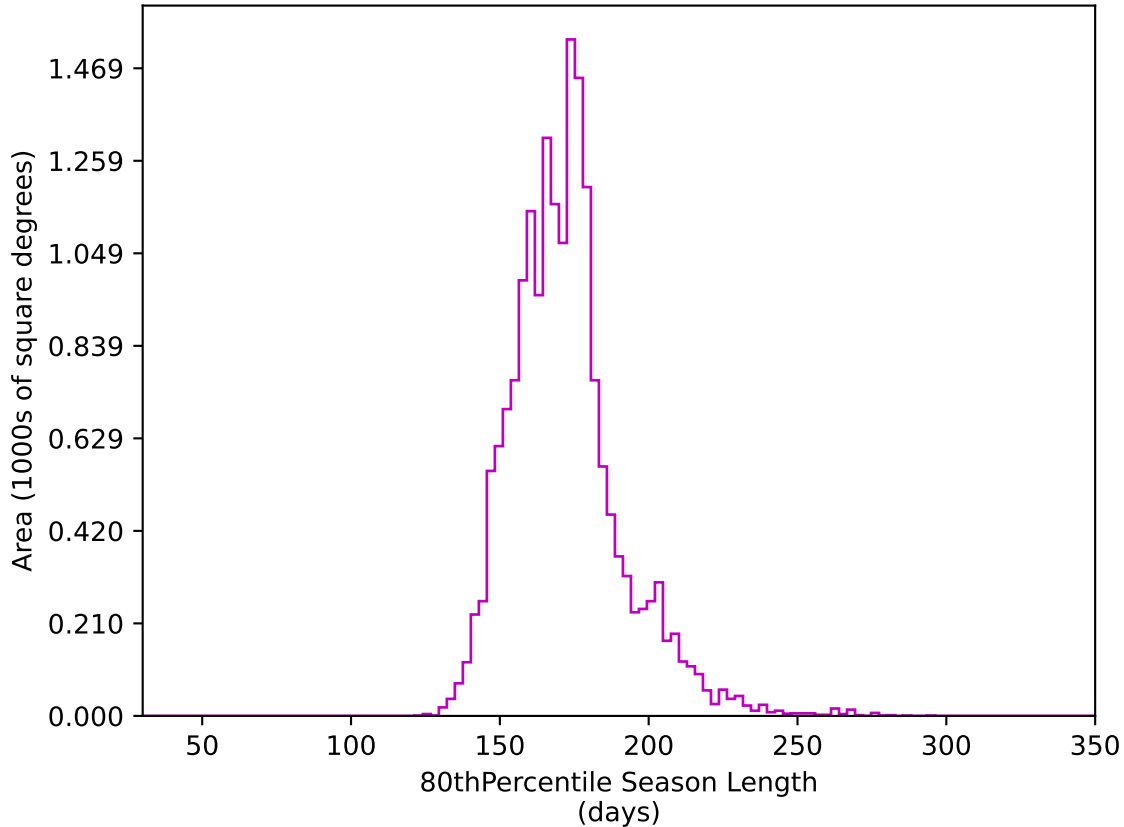
too_ignore_10_4v3.4_10yrs WFD z band: 80thPercentile Season Length
