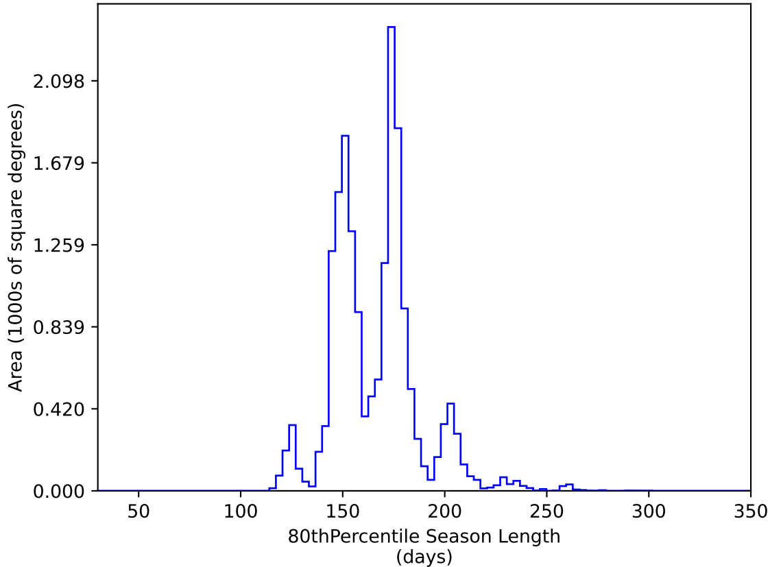
too_ignore_10_4v3.4_10yrs WFD y band: 80thPercentile Season Length
