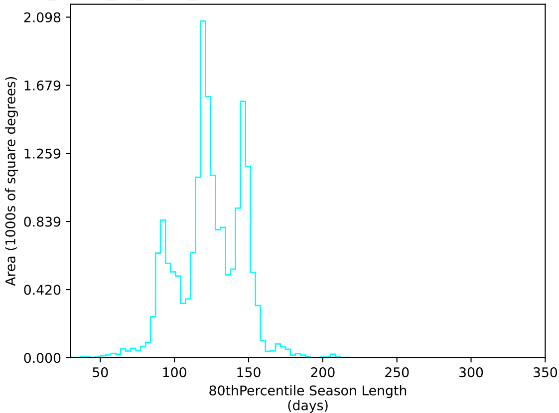
too_ignore_10_4v3.4_10yrs WFD u band: 80thPercentile Season Length
