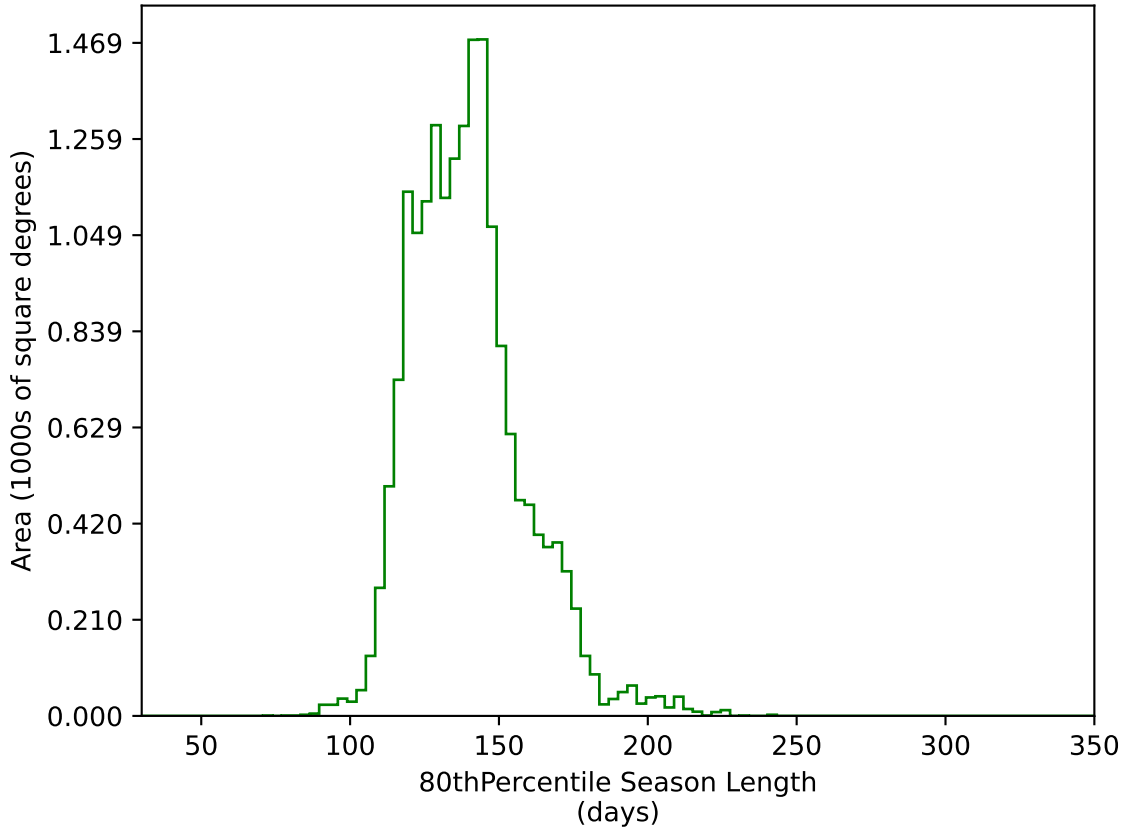
too_ignore_10_4v3.4_10yrs WFD g band: 80thPercentile Season Length
