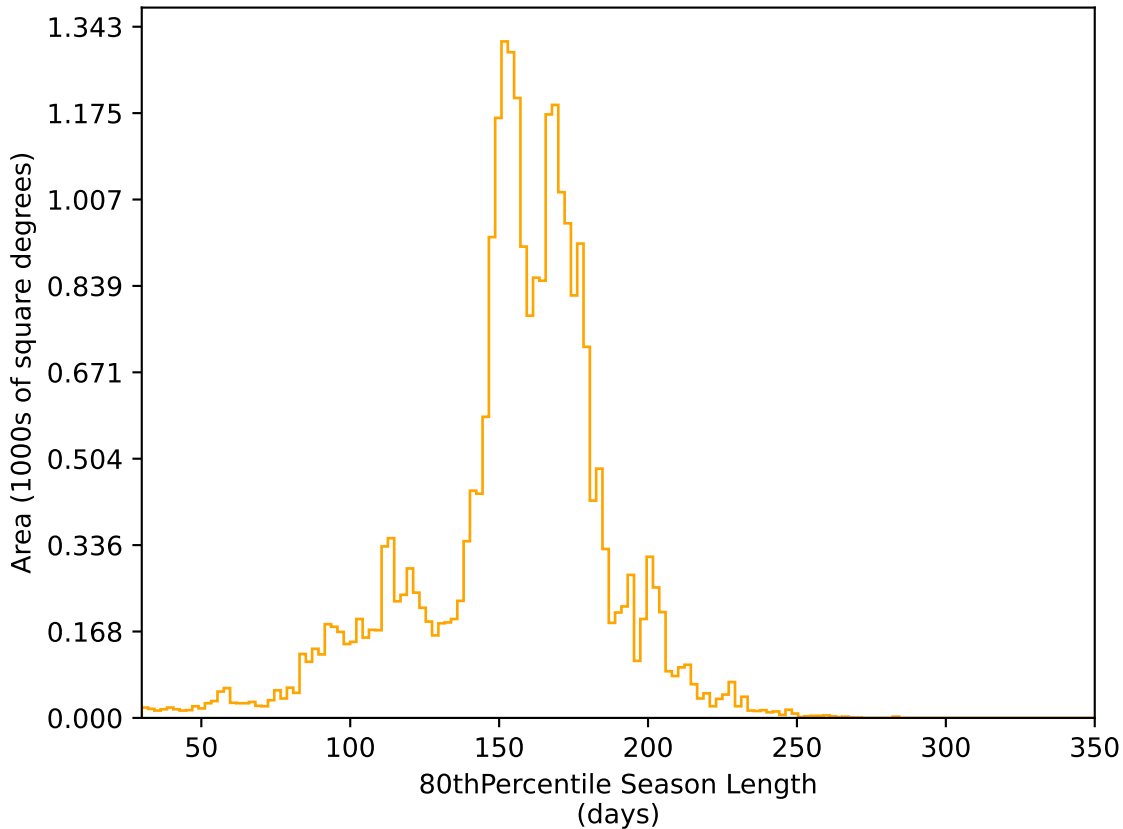
too_ignore_10_4v3.4_10yrs All sky r band: 80thPercentile Season Length
