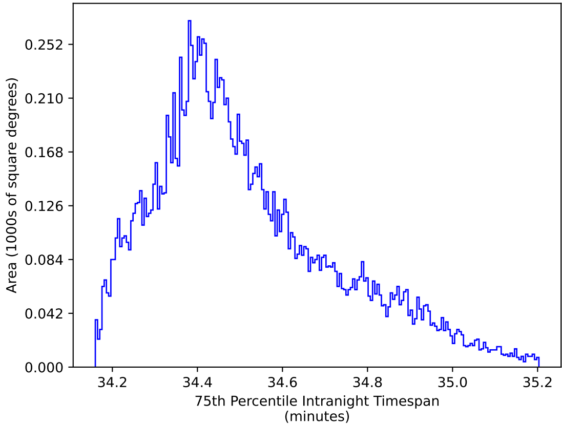
too_ignore_10_4v3.4_10yrs WFD zy bands: 75th Percentile Intranight Timespan
