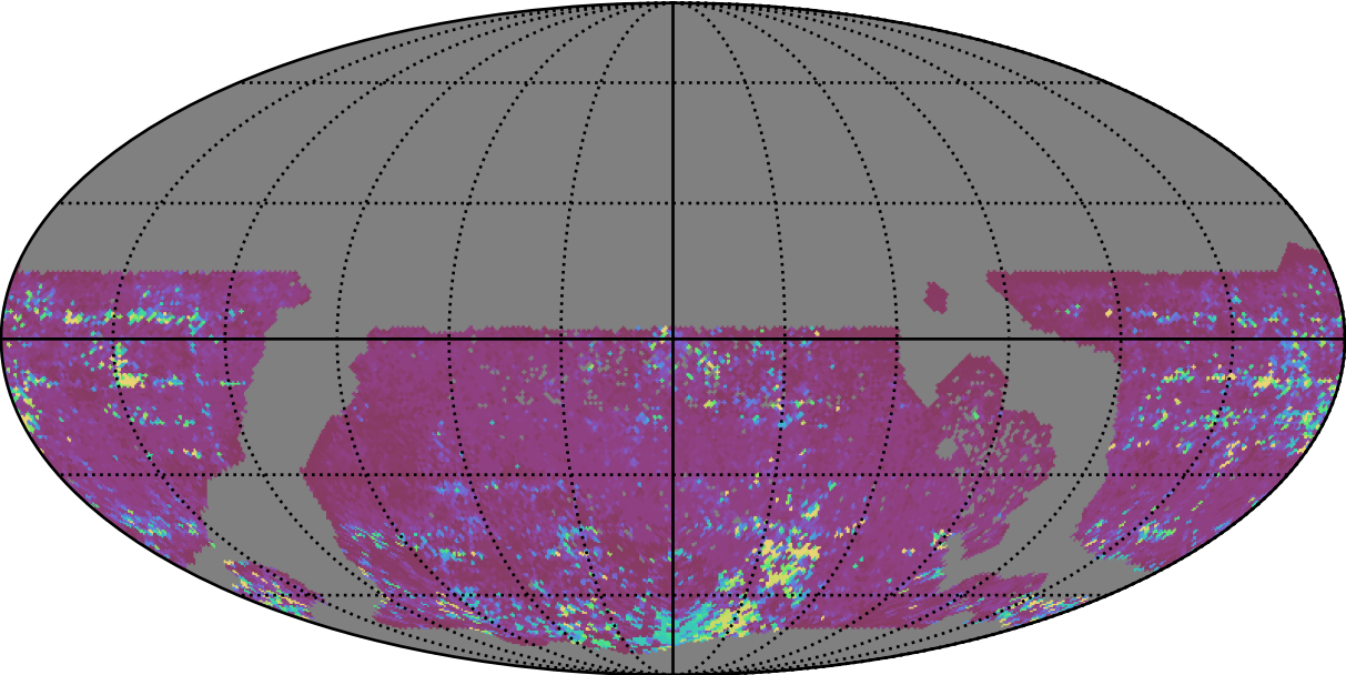
too_ignore_10_4v3.4_10yrs WFD z band: 75th Percentile Intranight Timespan
