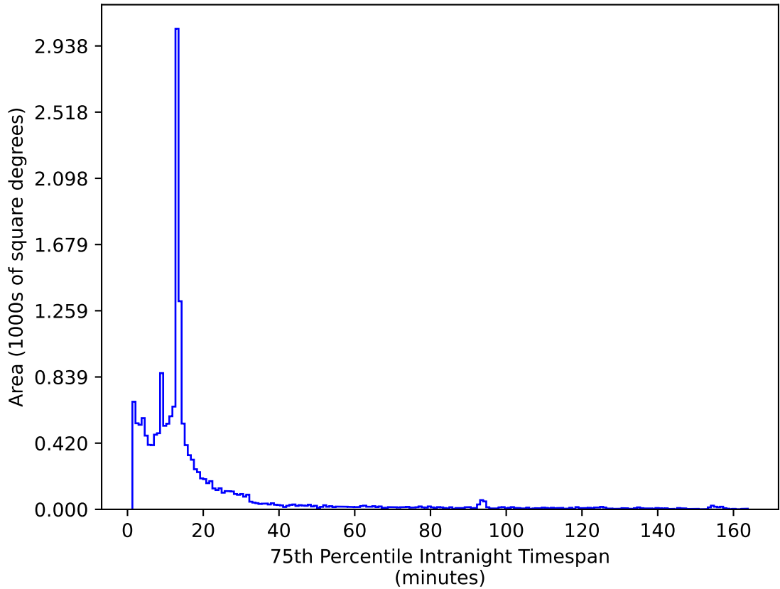
too_ignore_10_4v3.4_10yrs WFD z band: 75th Percentile Intranight Timespan
