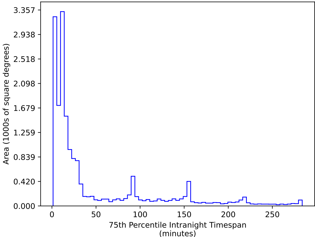
too_ignore_10_4v3.4_10yrs WFD r band: 75th Percentile Intranight Timespan
