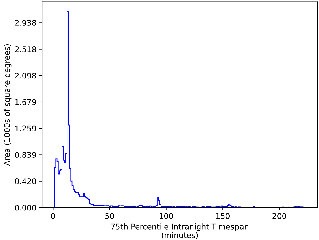
too_ignore_10_4v3.4_10yrs WFD i band: 75th Percentile Intranight Timespan
