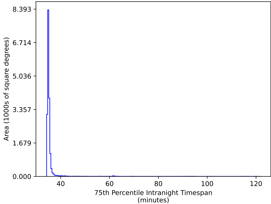
too_ignore_10_4v3.4_10yrs WFD gr bands: 75th Percentile Intranight Timespan
