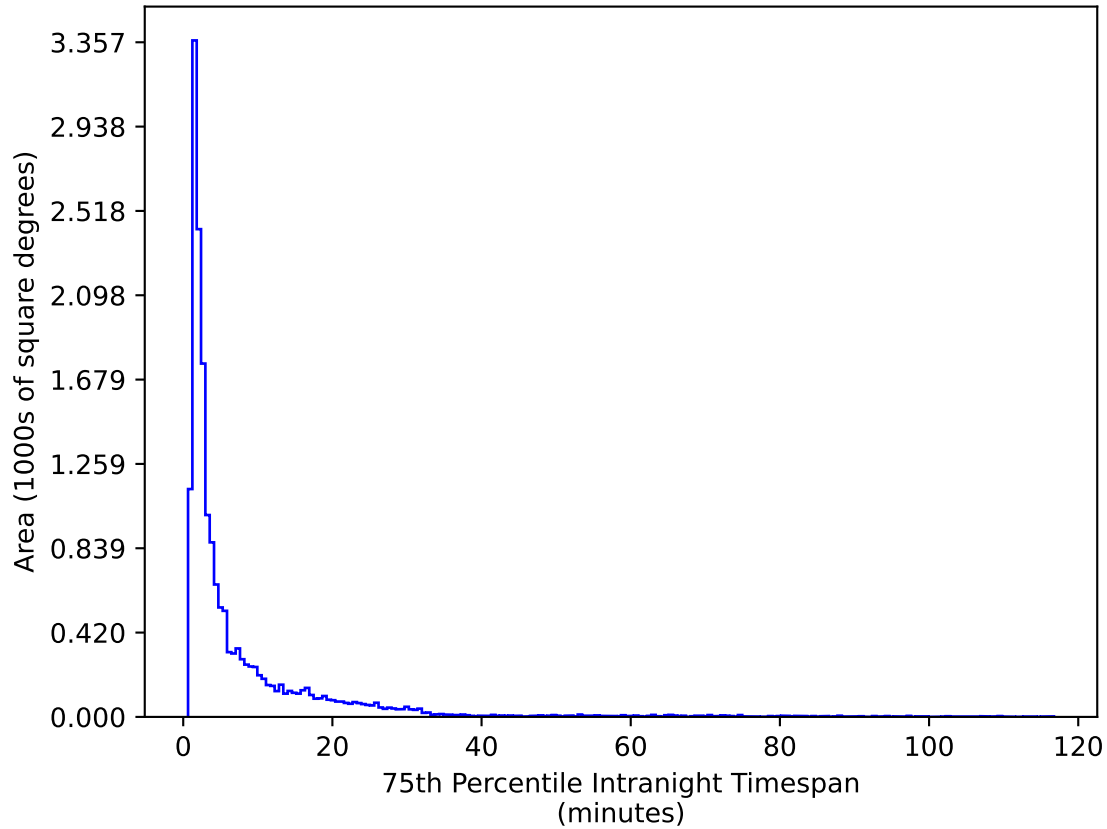
too_ignore_10_4v3.4_10yrs WFD g band: 75th Percentile Intranight Timespan
