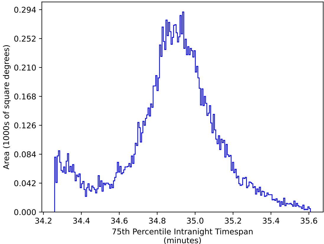
too_ignore_10_4v3.4_10yrs WFD all bands: 75th Percentile Intranight Timespan
