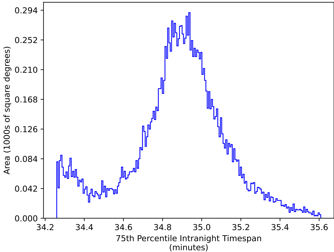
too_ignore_10_4v3.4_10yrs WFD: 75th Percentile Intranight Timespan
