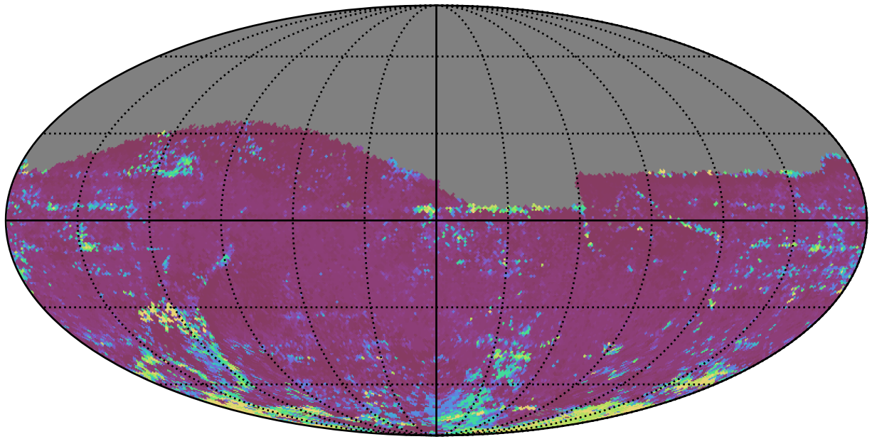
too_ignore_10_4v3.4_10yrs All sky z band: 75th Percentile Intranight Timespan
