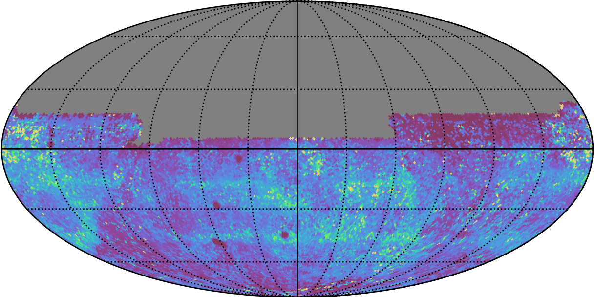
too_ignore_10_4v3.4_10yrs All sky y band: 75th Percentile Intranight Timespan
