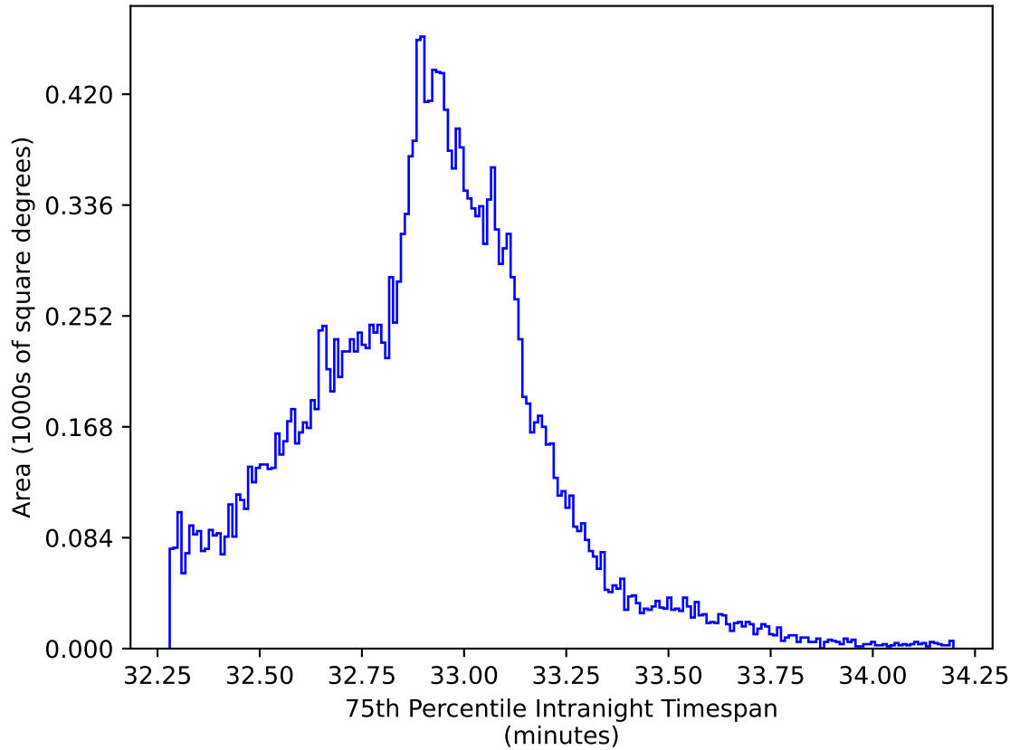
too_ignore_10_4v3.4_10yrs All sky y band: 75th Percentile Intranight Timespan
