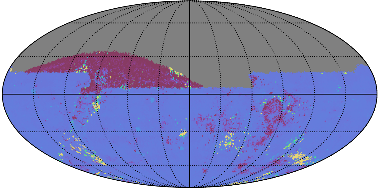
too_ignore_10_4v3.4_10yrs All sky ug bands: 75th Percentile Intranight Timespan
