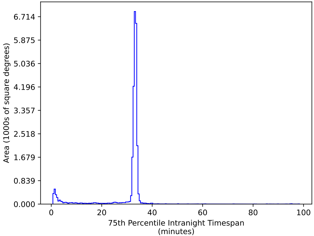
too_ignore_10_4v3.4_10yrs All sky ug bands: 75th Percentile Intranight Timespan
