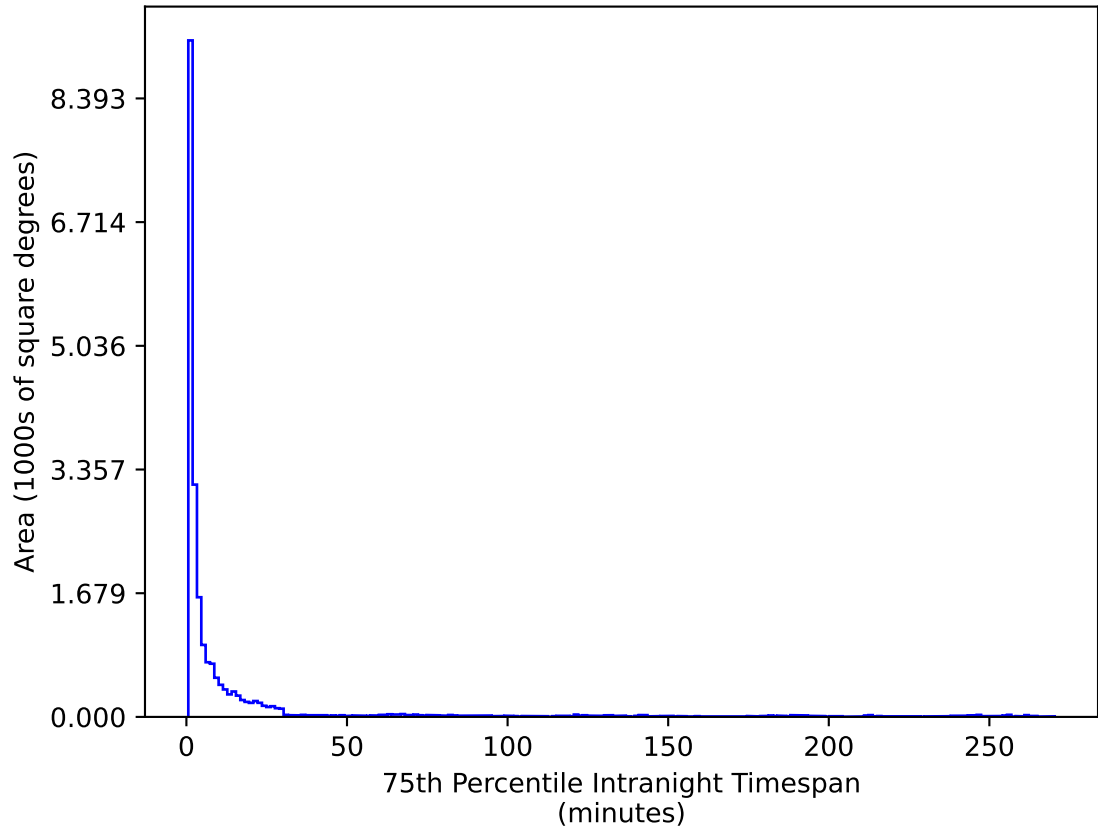
too_ignore_10_4v3.4_10yrs All sky u band: 75th Percentile Intranight Timespan
