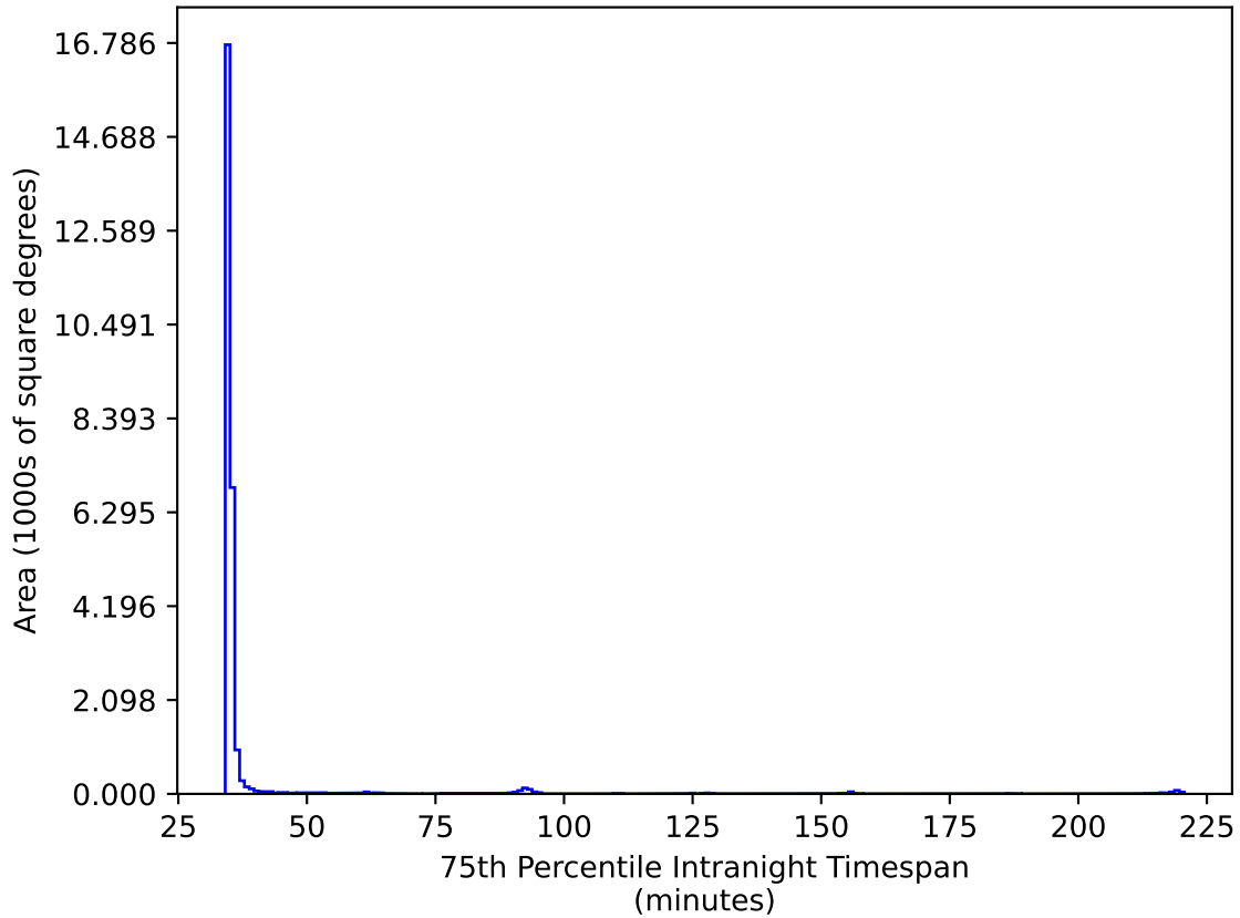
too_ignore_10_4v3.4_10yrs All sky ri bands: 75th Percentile Intranight Timespan
