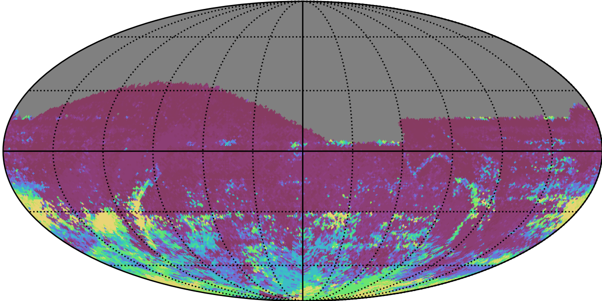
too_ignore_10_4v3.4_10yrs All sky r band: 75th Percentile Intranight Timespan
