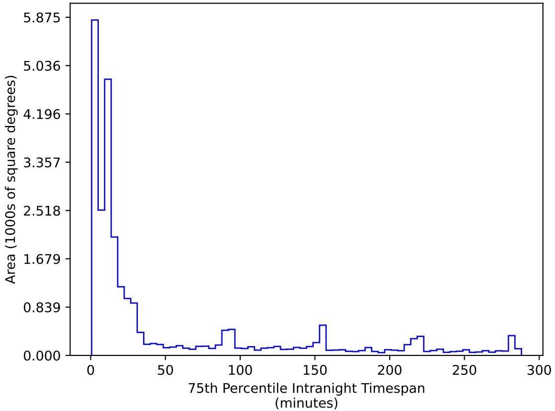
too_ignore_10_4v3.4_10yrs All sky r band: 75th Percentile Intranight Timespan
