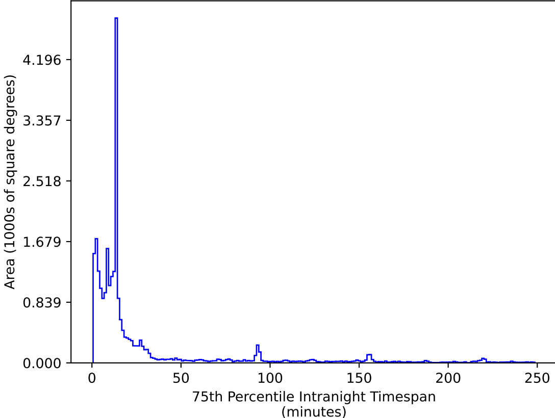
too_ignore_10_4v3.4_10yrs All sky i band: 75th Percentile Intranight Timespan
