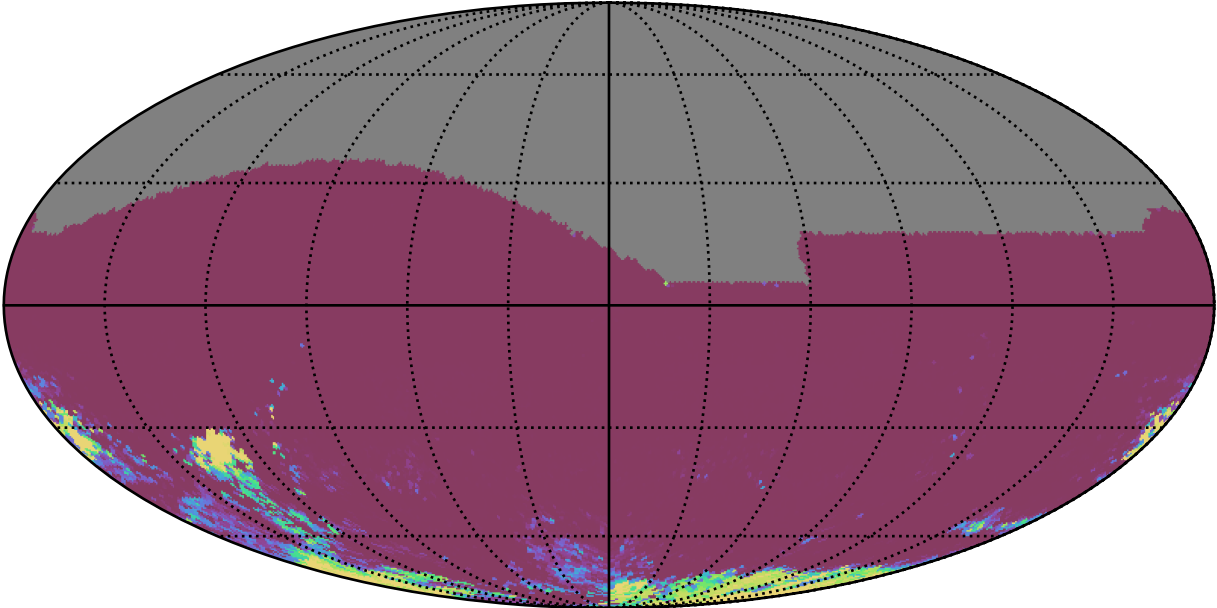
too_ignore_10_4v3.4_10yrs All sky gr bands: 75th Percentile Intranight Timespan
