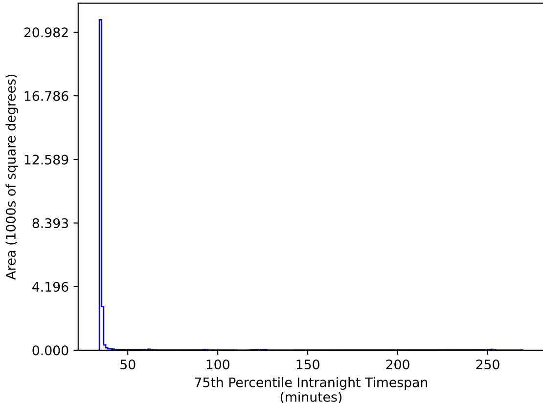
too_ignore_10_4v3.4_10yrs All sky gr bands: 75th Percentile Intranight Timespan
