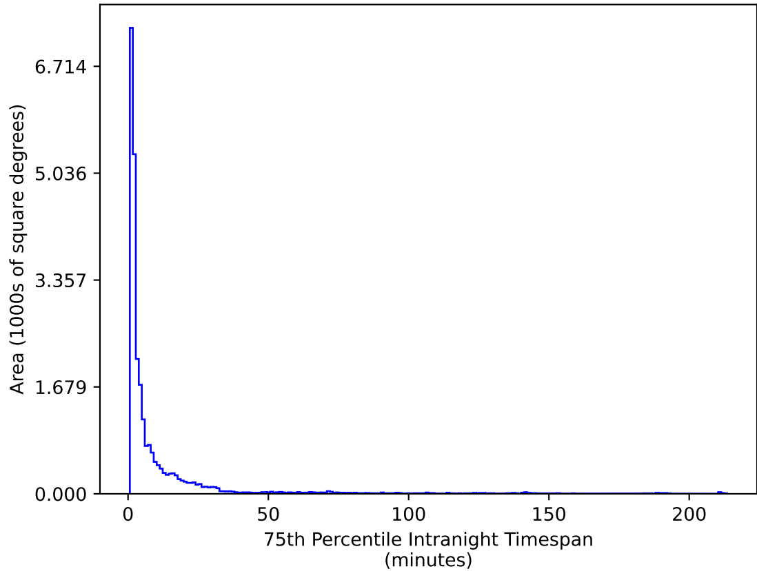
too_ignore_10_4v3.4_10yrs All sky g band: 75th Percentile Intranight Timespan
