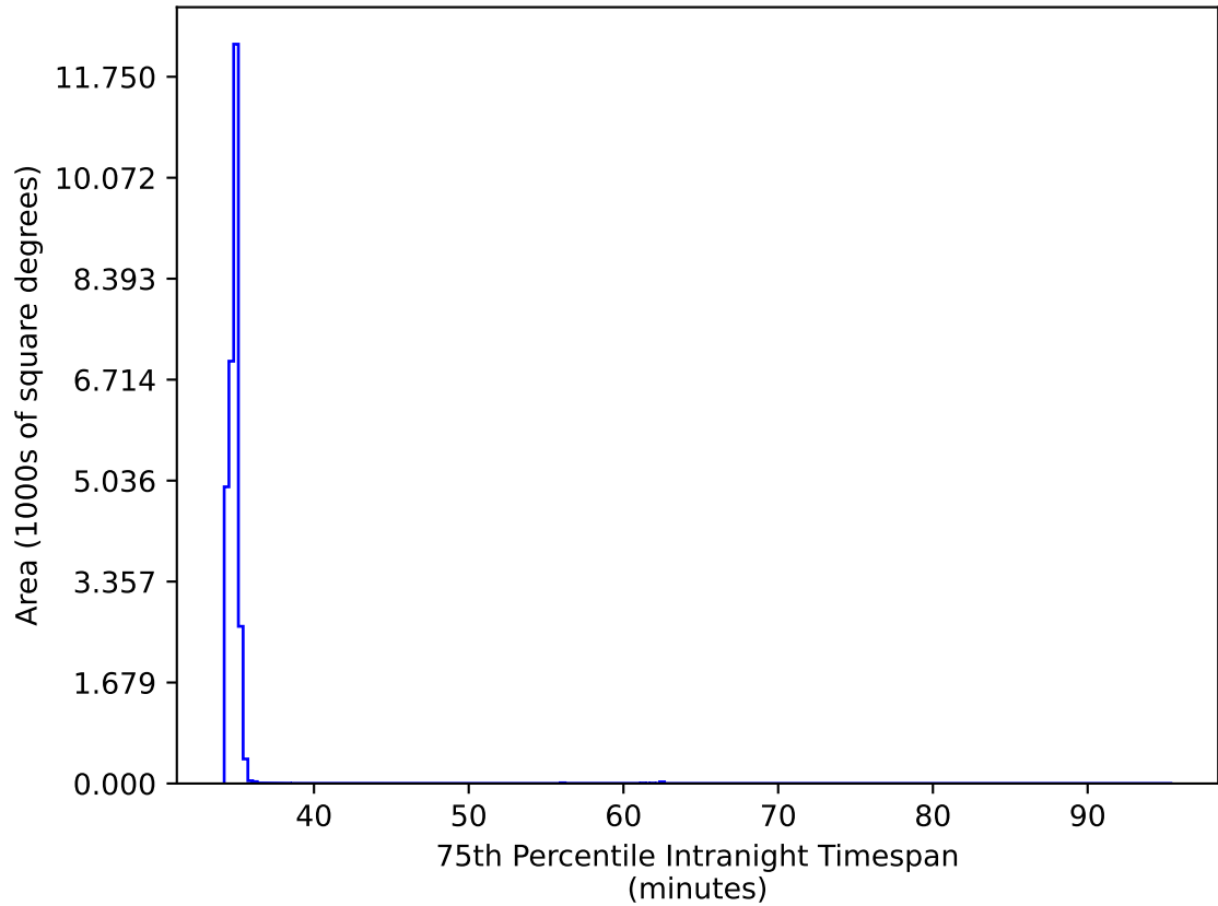
too_ignore_10_4v3.4_10yrs All sky all bands: 75th Percentile Intranight Timespan
